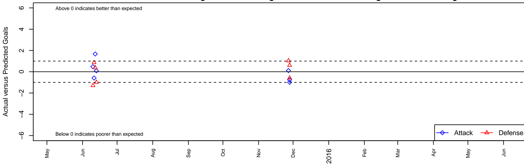
Cook Inlet Velocity Blue B99 Dots are actual minus expected GF (blue circles) and GA (red triangles). Blue line is smoothed change in attack strength. Red is smoothed change in defense strength.
